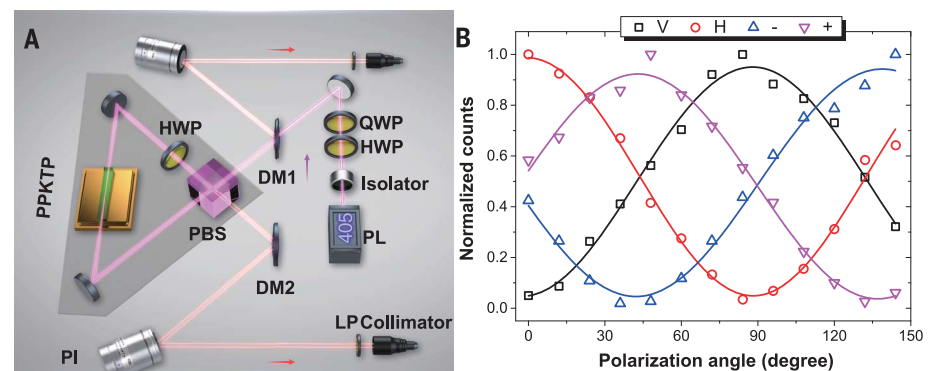
Fig. 1. Schematic of the spaceborne entangled-photon source and its in-orbit performance.
